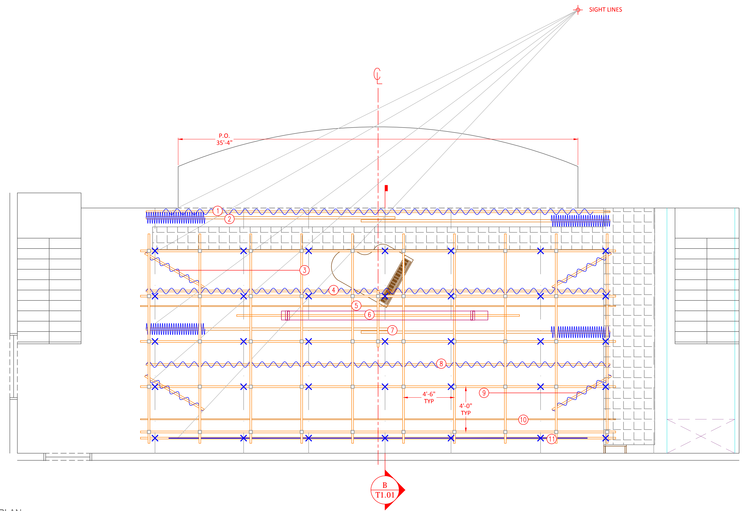
STAGE PLAN SCALE 1/4" = 1'-0"
