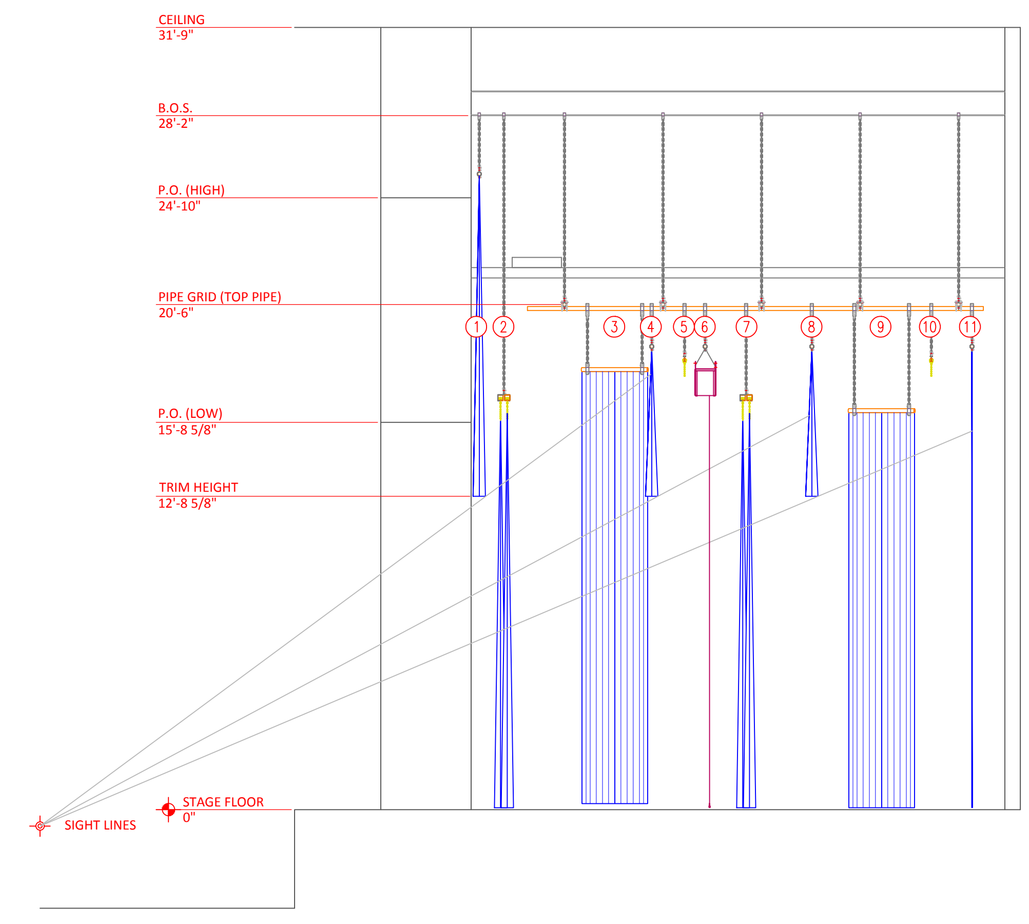
STAGE SECTION SCALE 1/4" = 1'-0"
